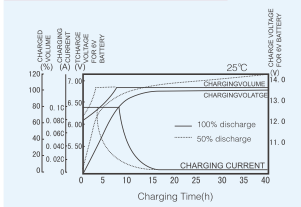
NP series Charging Characteristics
