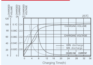
GM series Charging Characteristics
