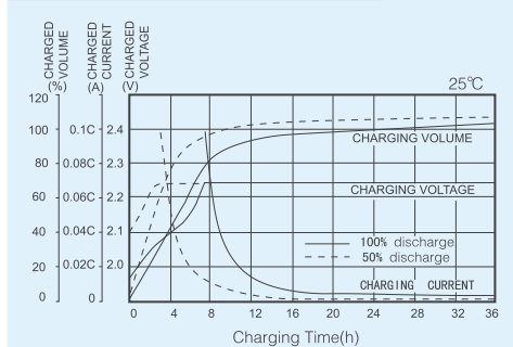
GM series Charging Characteristics
