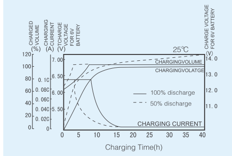
NP series Charging Characteristics
